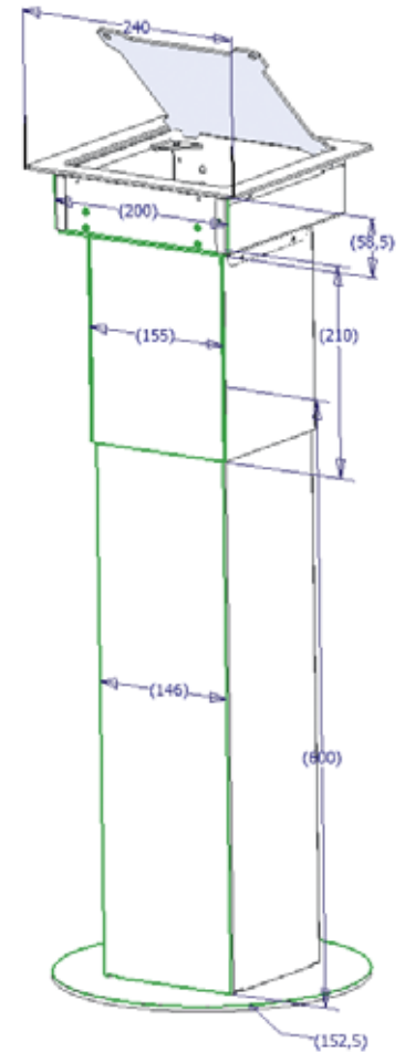
Detail drawing: Skytower with option tower and base
