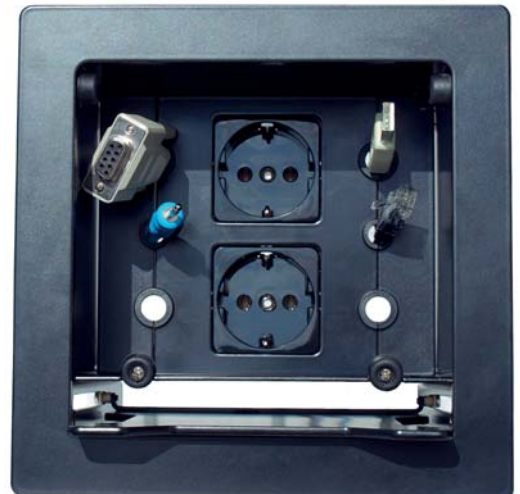
AF-TA Sky KCC-S6 with standard surface black powdered Inside view with sample mounting and fold-in cover
